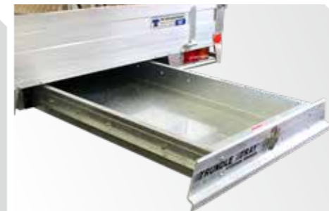
Trundle Tray™ to suit Dual Cab (1500mm), King Cab (1800mm) or Single Cab (2100mm)
